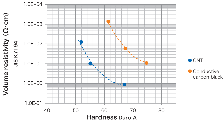
Figure 1. Relationship between hardness and volume resistivity
